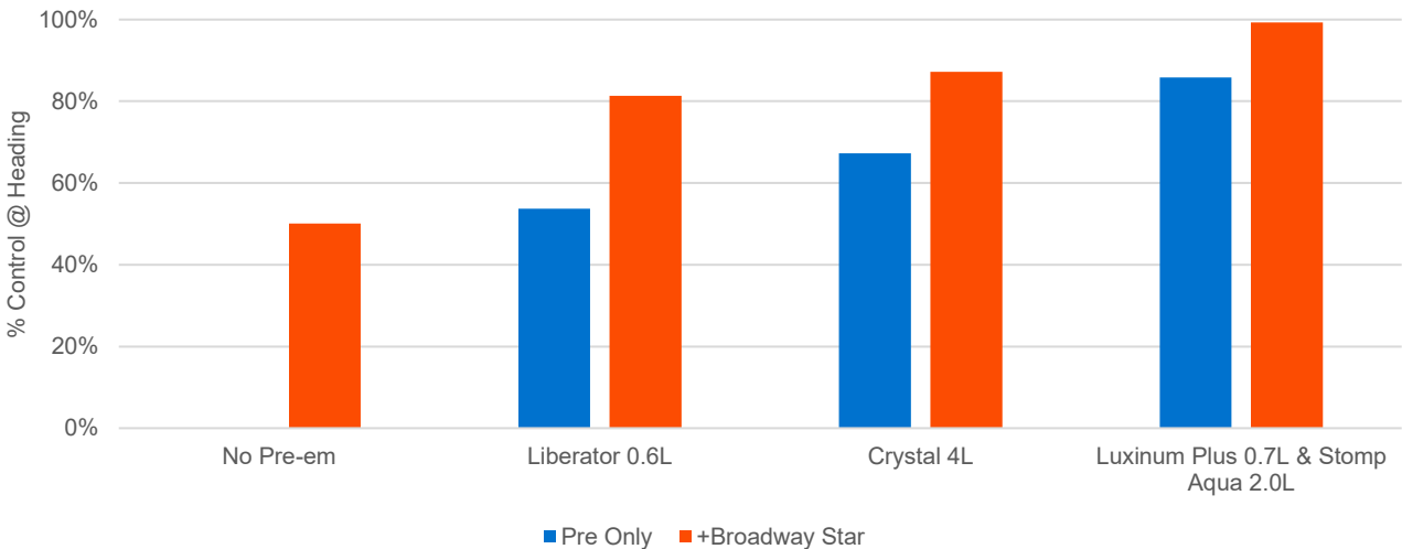
Mean of 4 Corteva trials on LOLMU, pre-emergence application followed by Broadway Star in spring.
